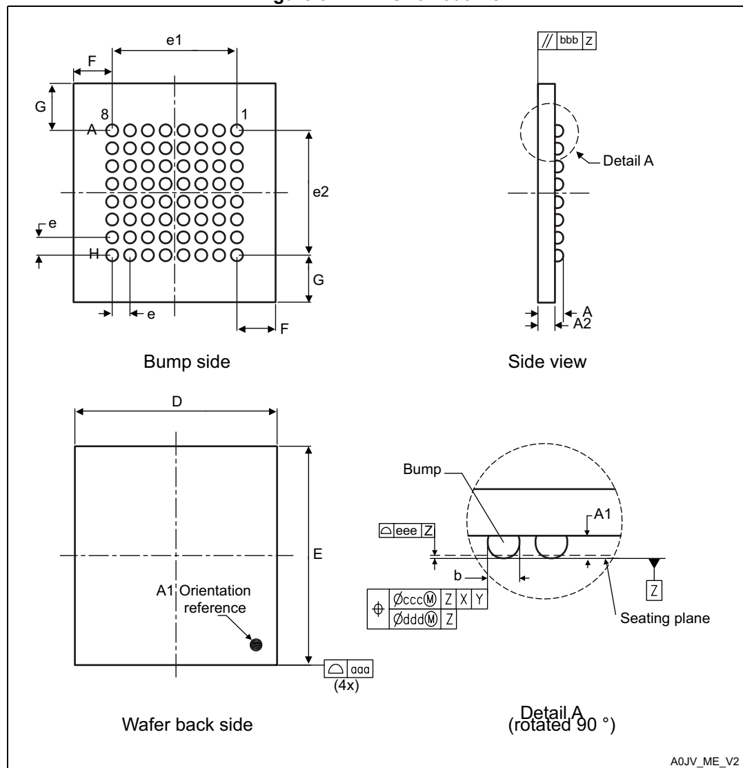
Figure 34. WLCSP64 outline
