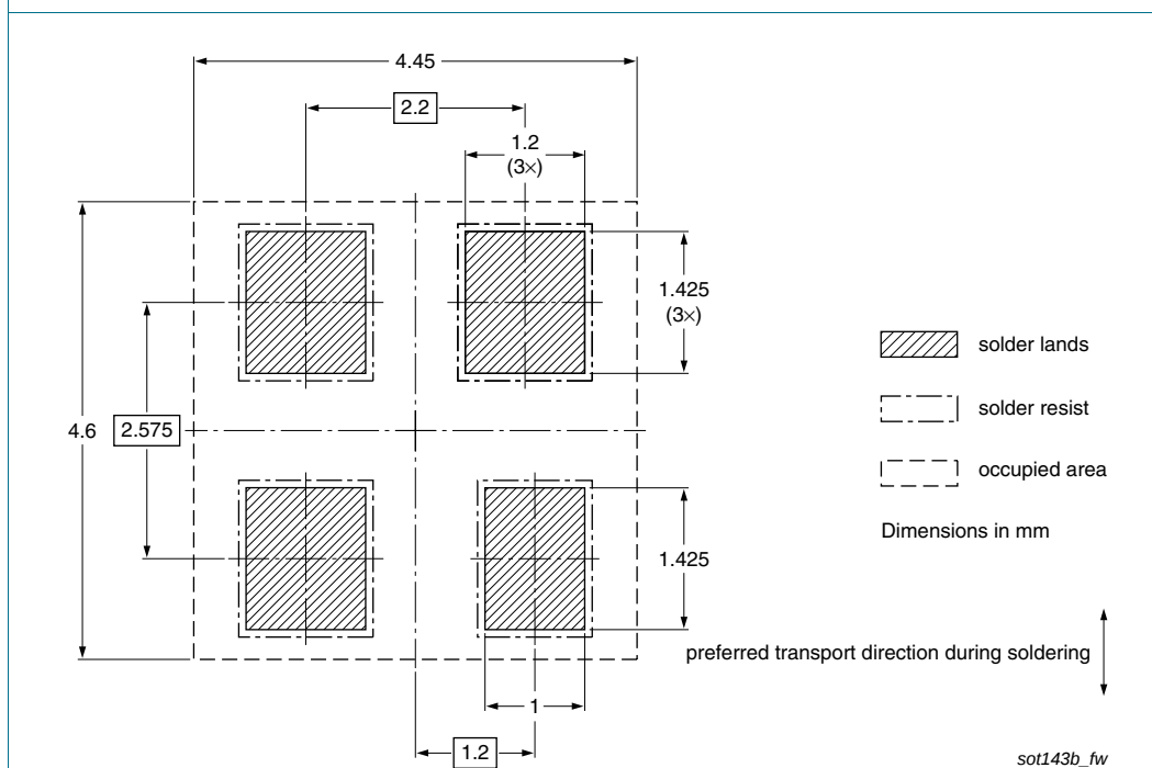
Fig 10. Wave soldering footprint BAS56 (SOT143B)
