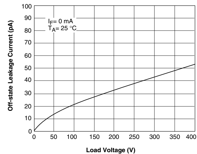
Figure 5. Leakage Current vs. Applied Voltage
