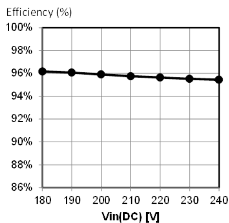
Figure 21. Efficiency vs. Vin(DC) (LED Vf=90V)
