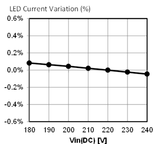
Figure 18. LED Current Ratio vs. Vin(DC) (Reference: Vin=220V, LED Vf=90V)
