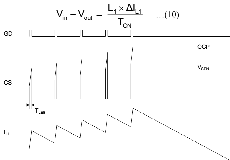
Figure 6. Peak Current Error by the Shortest ON Time (Shortest ON Time < T_{LEB} )
