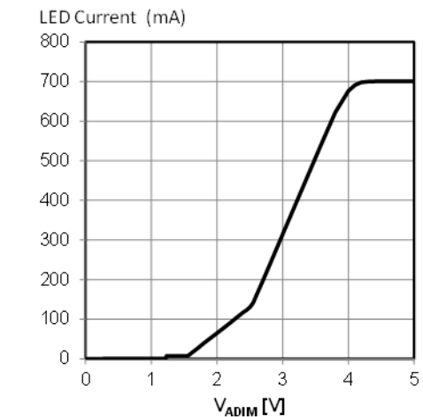
Figure 22. Complex Dimming Performance (VADIM)
