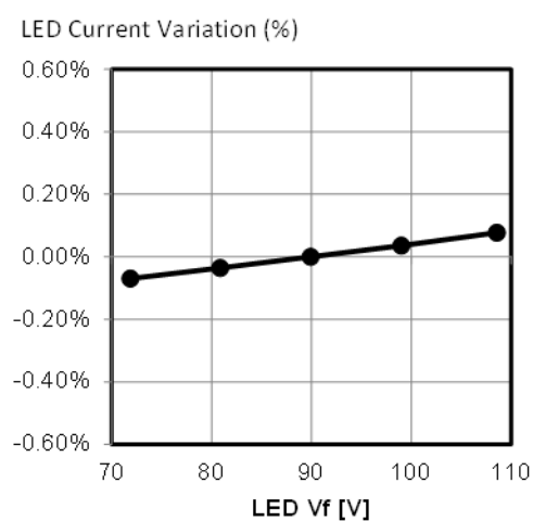
Figure 20. LED Current Ratio vs. LED Vf (Reference: Vin=220V, LED Vf=90V)
