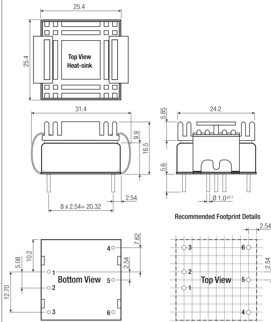
Dimension Drawing (mm) with Heat-sink
