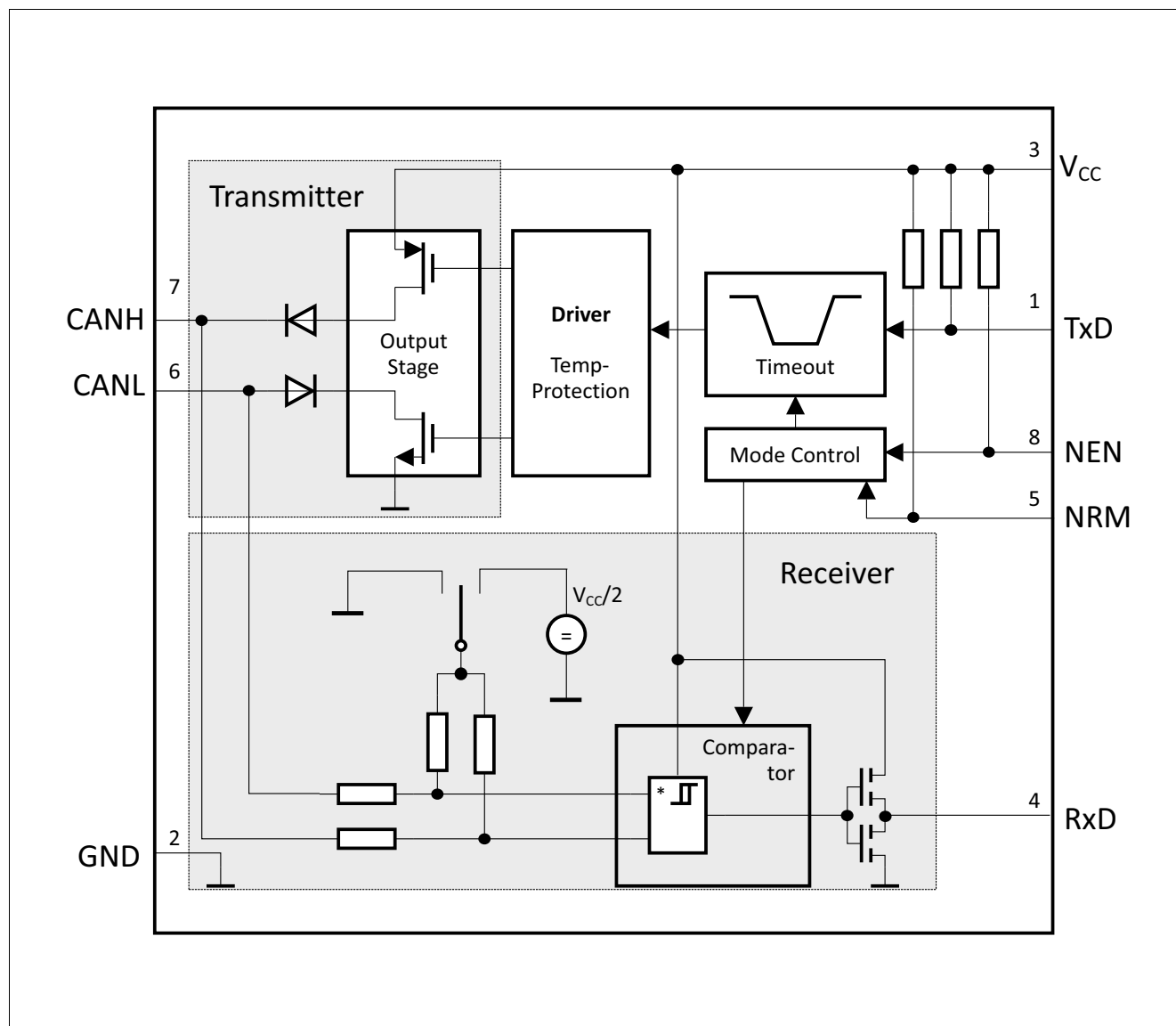
Figure 1 Block diagram
