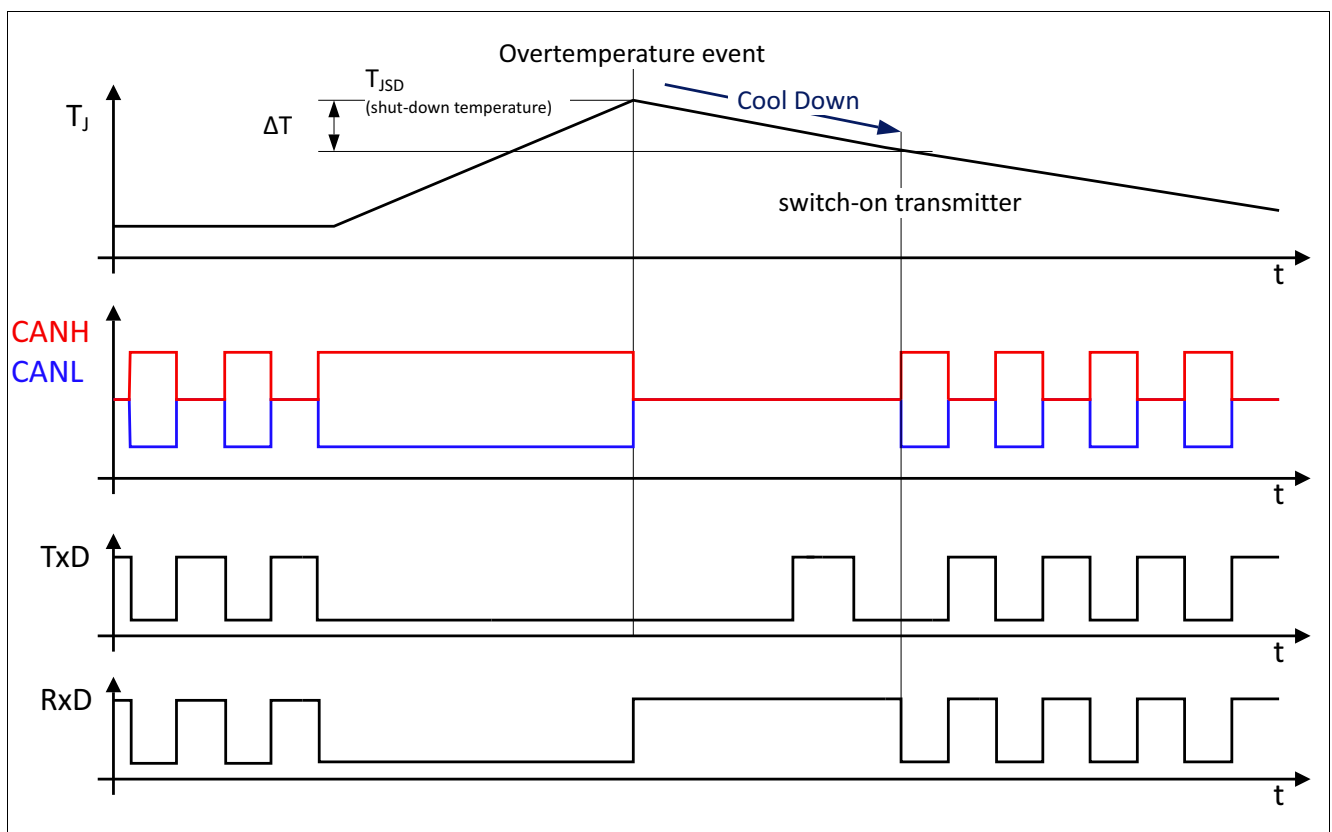
Figure 7 Overtemperature protection
