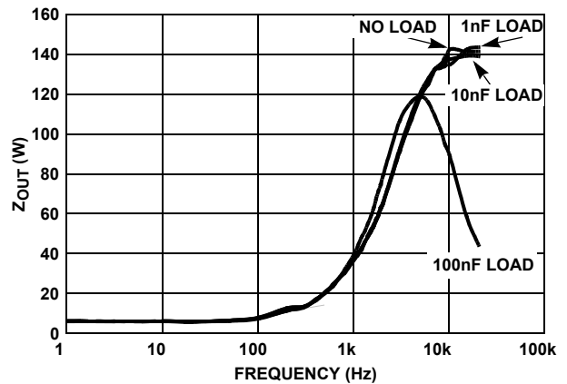
FIGURE 114. Z_{OUT} vs FREQUENCY
