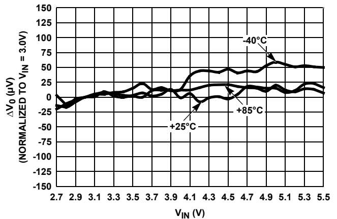
FIGURE 46. LINE REGULATION OVER-TEMPERATURE
