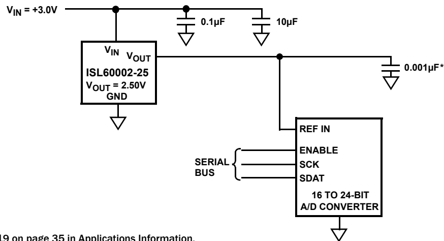
FIGURE 1. TYPICAL APPLICATION
