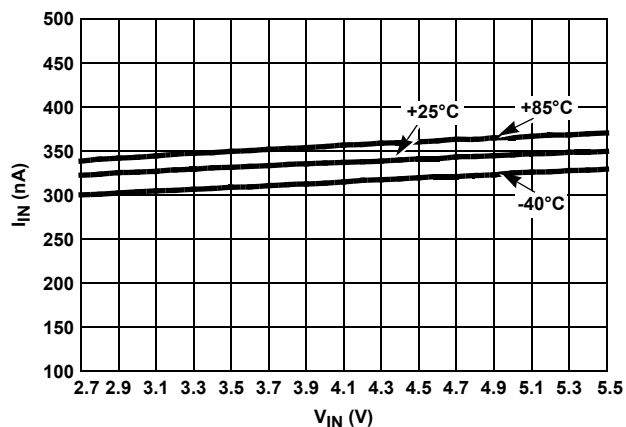
FIGURE 58. I_{IN} vs V_{IN} OVER-TEMPERATURE
