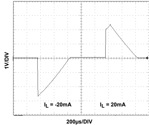
FIGURE 112. LOAD TRANSIENT RESPONSE
