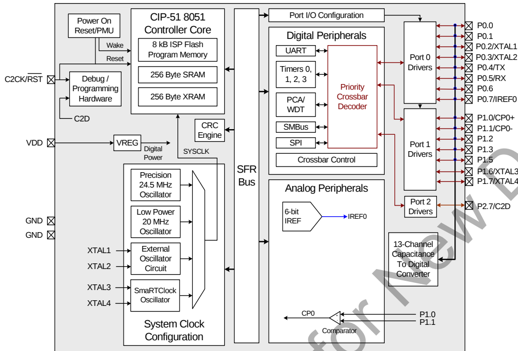
Figure 1.11. C8051F991 Block Diagram
