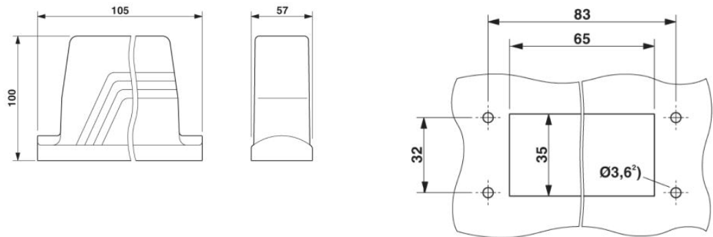
Dimensioned drawing
