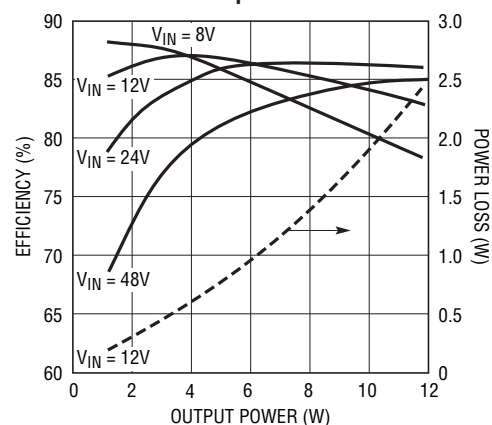
Efficiency and Power Loss vs Output Power
