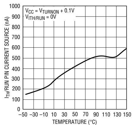
I_{TH}/RUN Start-Up Current Source vs Temperature
