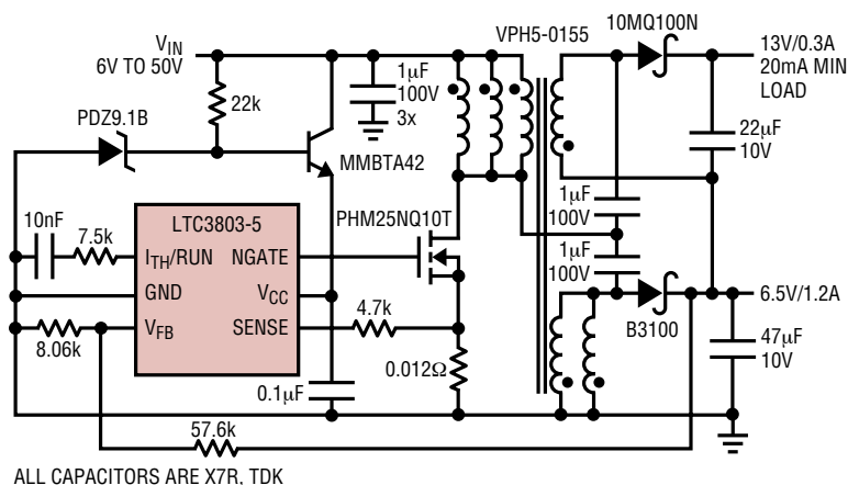
Dual Output Wide Input Range Converter
