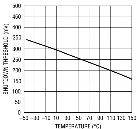
I_{TH}/RUN Shutdown Threshold vs Temperature
