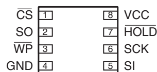
Figure 2-2. 8-UDFN (Top View)
