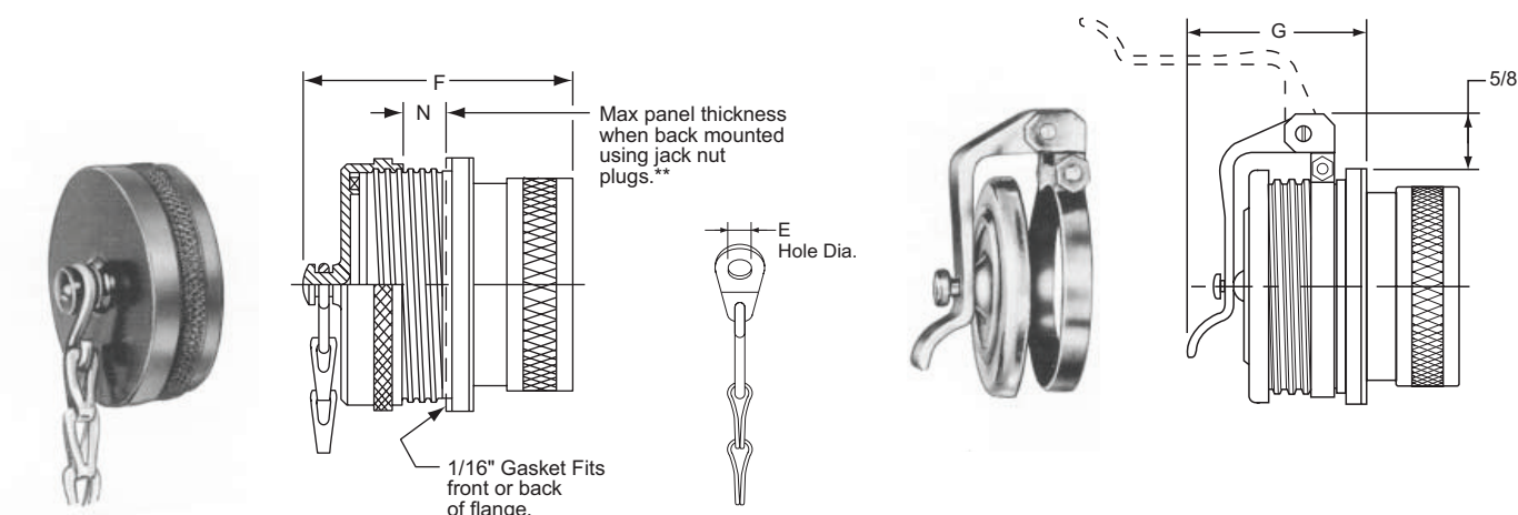
WITH THREADED ENVIRONMENTAL COVER AND SASH CHAIN
