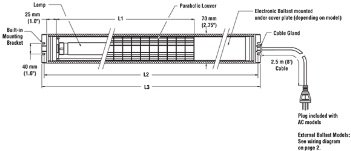
Figure 1. Dimensions for Models with Lamps 24 inches and Longer
