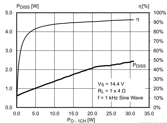
Figure 4. Efficiency and power dissipation ( V_S = 14.4 V, R_L = 1 \times 4 \Omega , f = 1 kHz sine wave)
