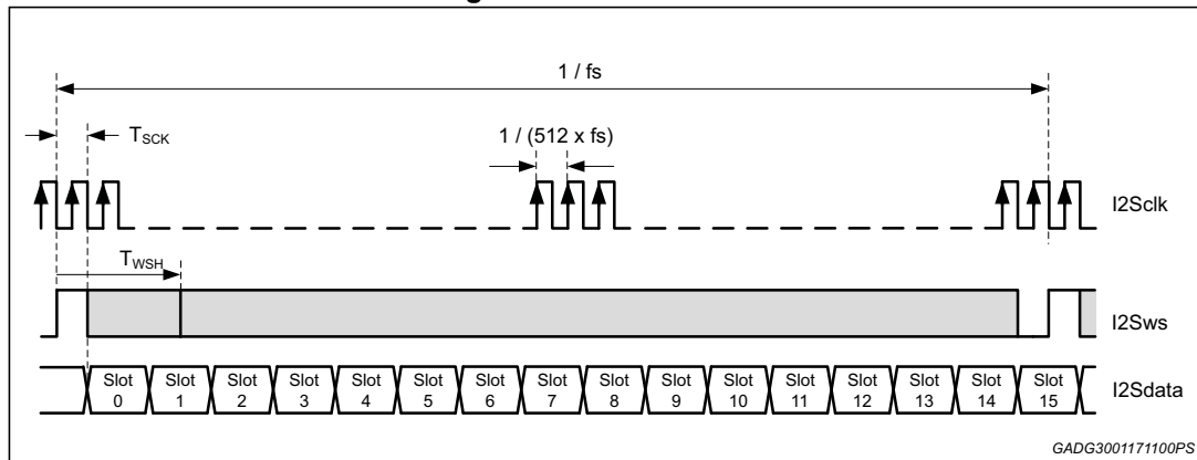
Figure 70. TDM16 mode
