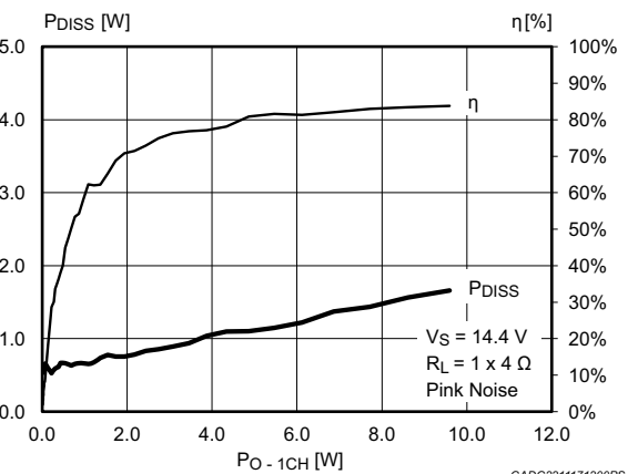
Figure 5. Efficiency and power dissipation ( V_S = 14.4 V, R_L = 1 \times 4 \Omega , pink noise)
