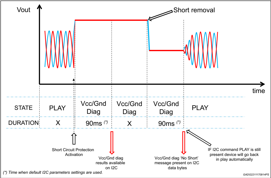
Figure 53. Short circuit protection activation - Short to VCC
