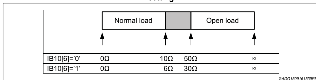
Figure 55. Open load in play detector guaranteed thresholds with standard gain setting
