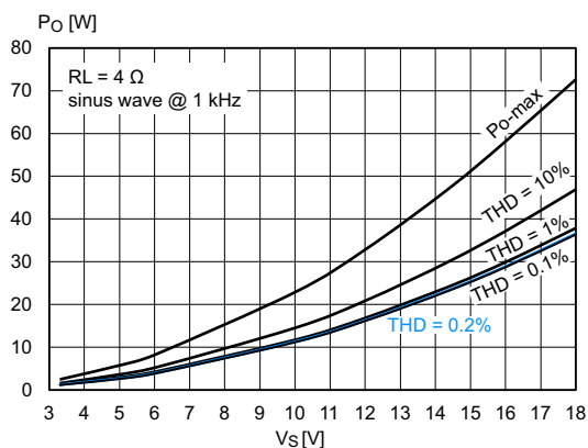
Figure 22. Output power vs. supply voltage ( R_L = 4\ \Omega , sine wave)
