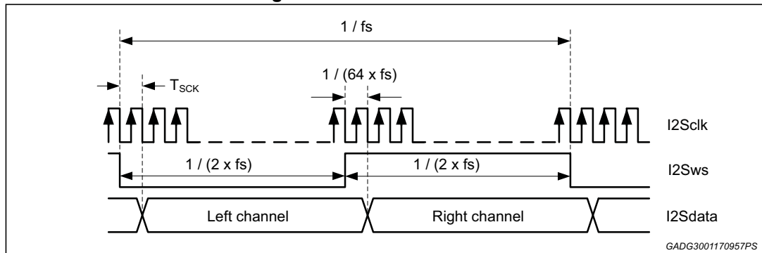
Figure 67. I 2 S standard mode
