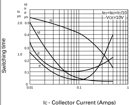
Switching Speeds
