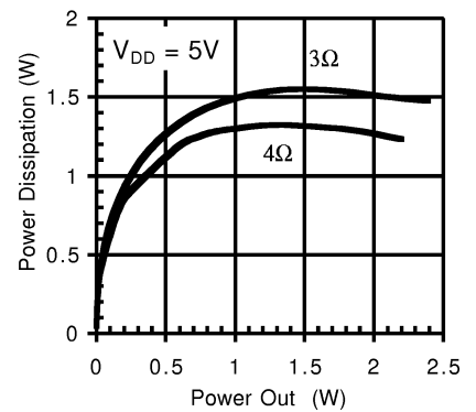
LM4873MTE, LM4873LQ Power Dissipation vs Power Output
