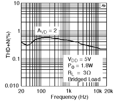
LM4873MTE, LM4873LQ THD+N vs Frequency
