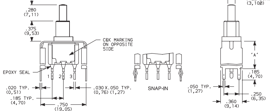
8161SH9_BE2 SPDT
