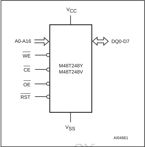
Figure 2. Logic Diagram
