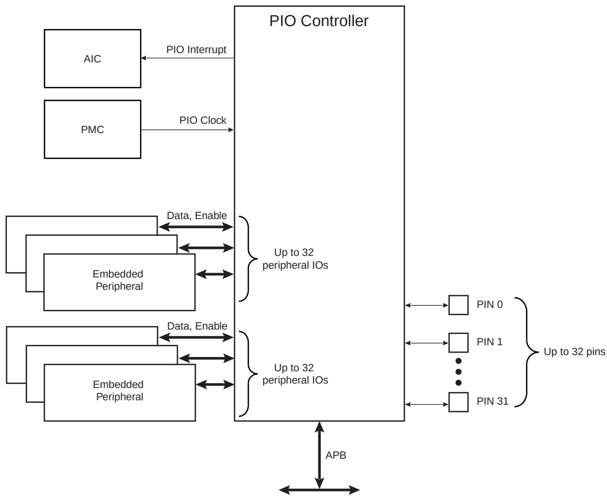
Figure 27-1. Block Diagram
