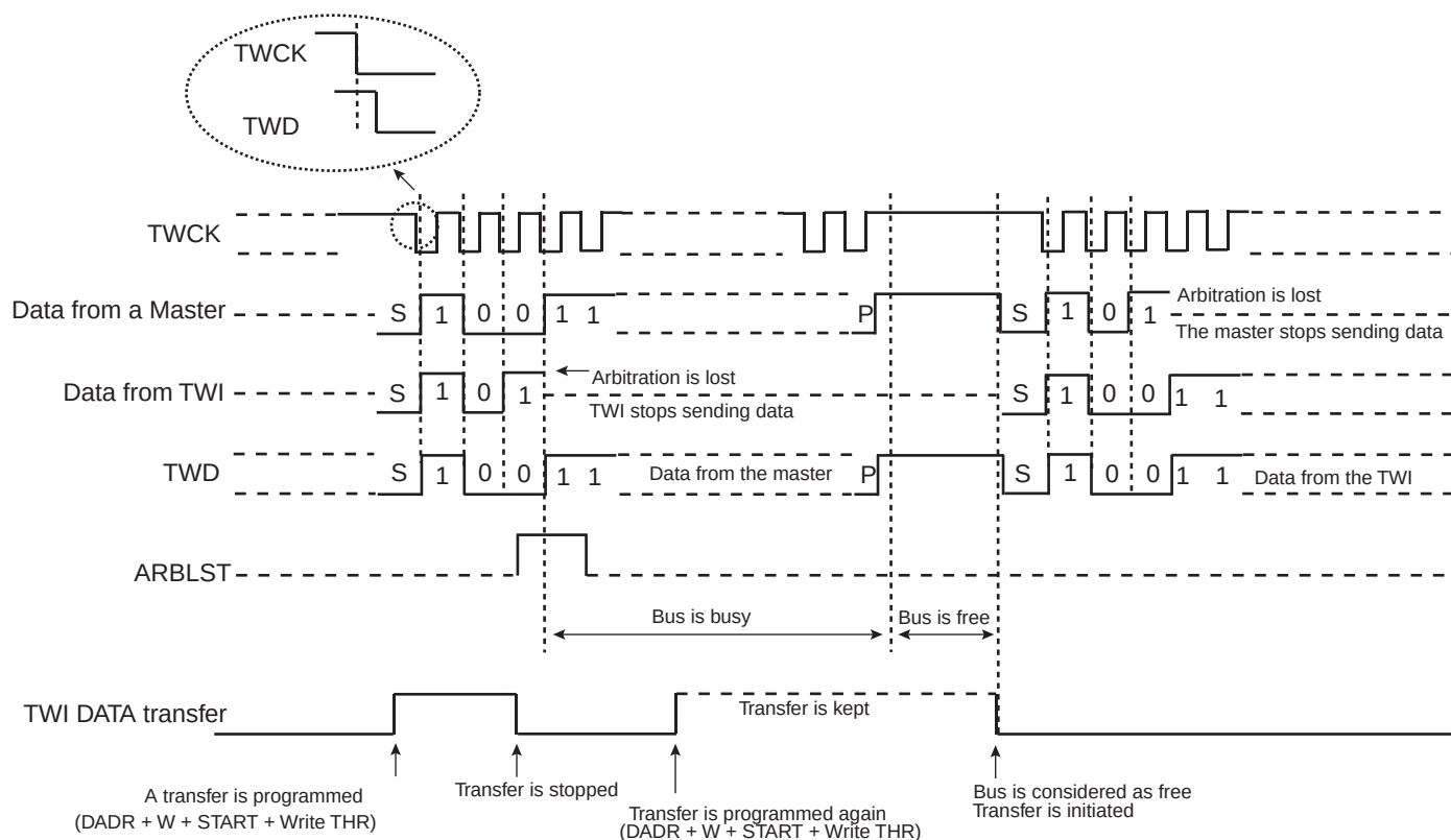
Figure 30-21. Arbitration Cases
