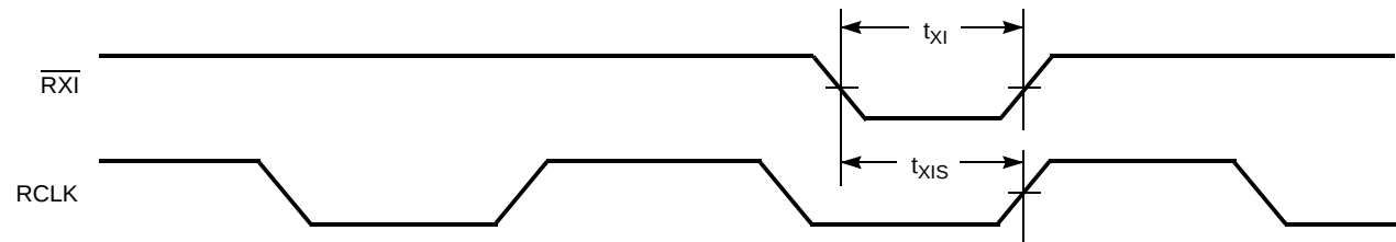
Figure 23. Retransmit Timing [37, 38, 39]
