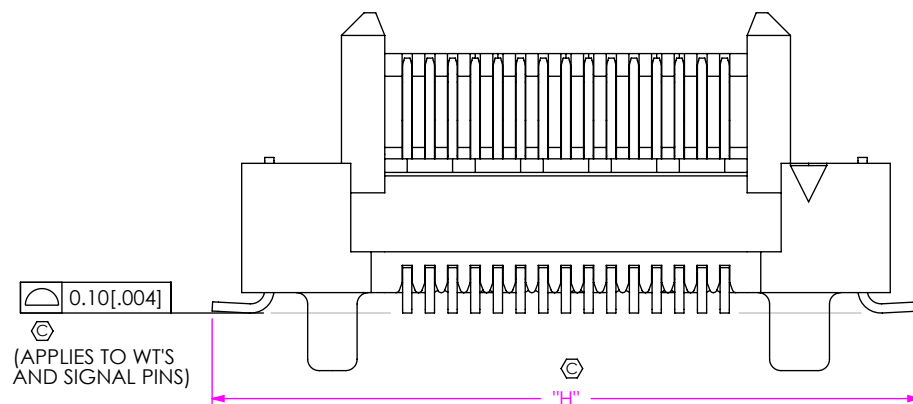
FIG 2 -SM WELD TAB (FT5-15-03.0-X-DV-SM-X-TR SHOWN) (SAME AS FIG 1, EXCEPT AS SHOWN) (NOT TOOLED)
