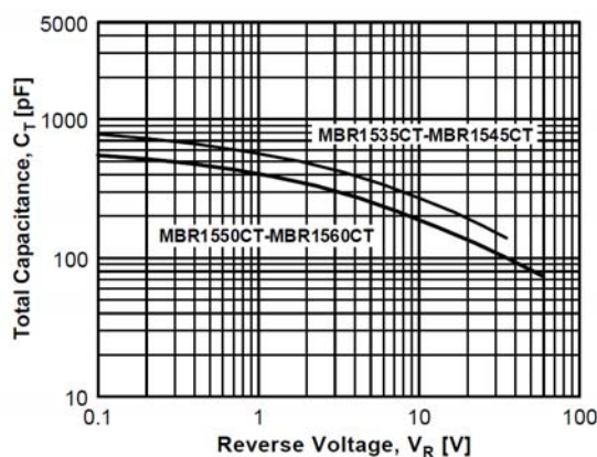
Figure 5. Total Capacitance
