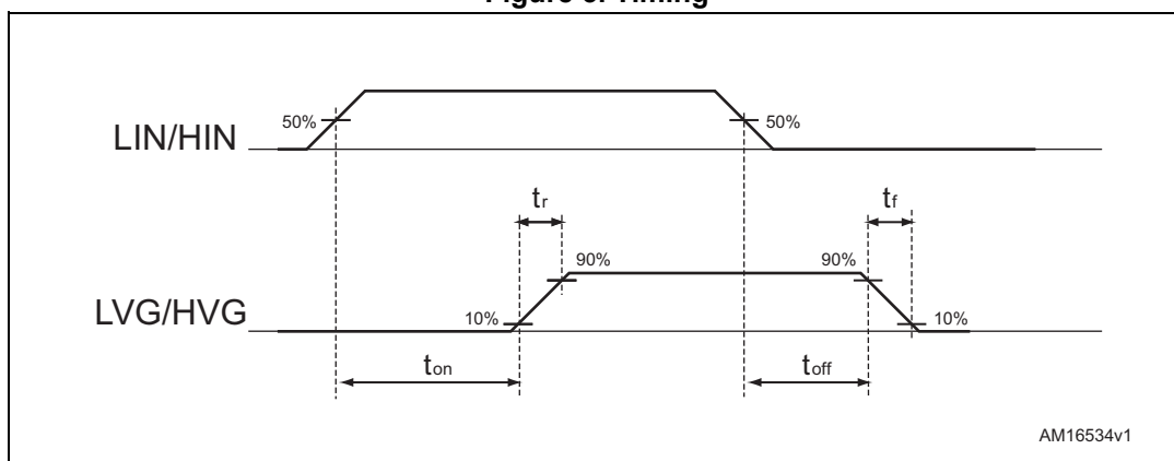
Figure 3. Timing
