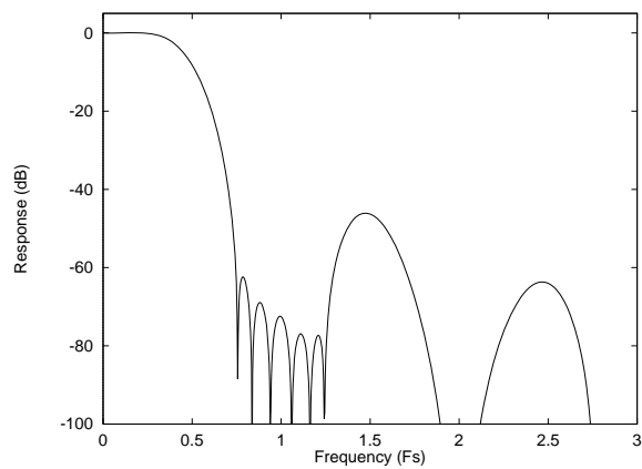
Figure 25 ADC Digital Filter Frequency Response – Type D
