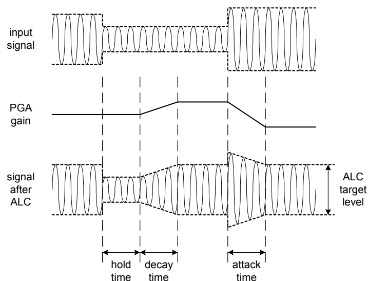
Figure 8 ALC Operation
