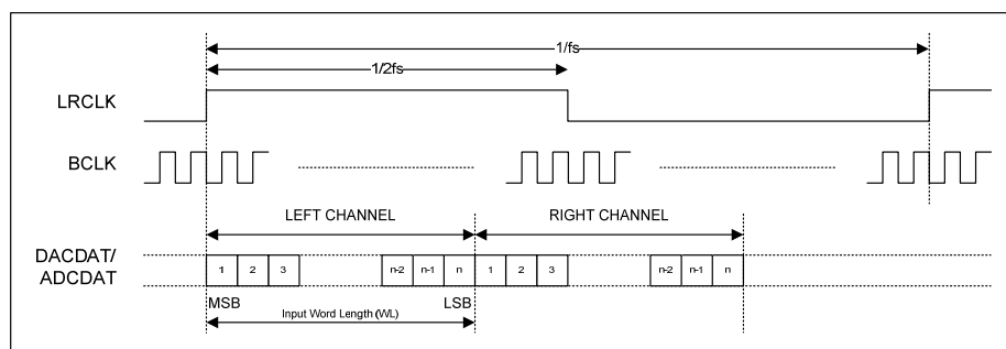
Figure 14 DSP Mode B, Master Mode Audio Interface
