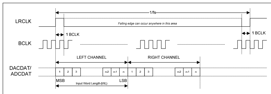
Figure 16 DSP Mode B Slave Mode
