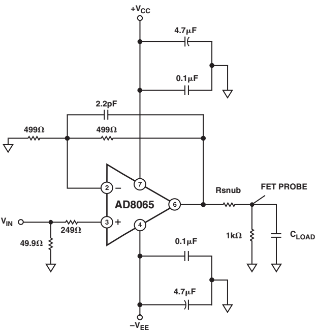
Test Circuit 2. G = +2
