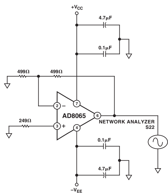
Test Circuit 6. Output Impedance G = +2
