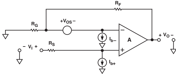
Figure 4. Voltage Feedback Amplifier DC Errors
