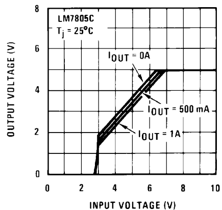
Dropout Characteristics
