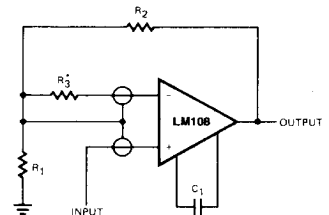
NON-INVERTING AMPLIFIER
