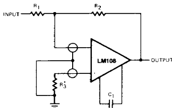
LIC-671 INVERTING AMPLIFIER
