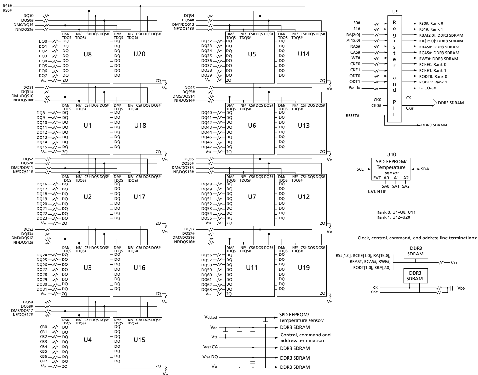
Figure 2: Functional Block Diagram
