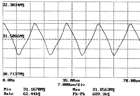
Figure 7. CY25819 Spread Spectrum Profile (Frequency vs. Time) [2]
