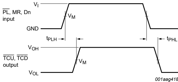
Measurement points are given in Table 10 . V_{OL} and V_{OH} are typical voltage output levels that occur with the output load.
