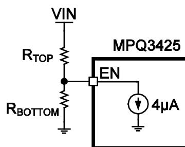
Figure 2: UVLO Hysteresis
