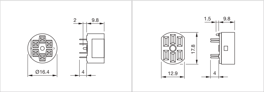
Dimensions [mm] for Part No. 31-940 Dimensions [mm] for Part No. 31-942
