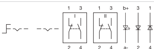
Wiring diagram 282
