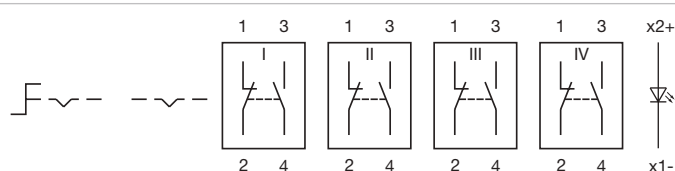
Wiring diagram 280
