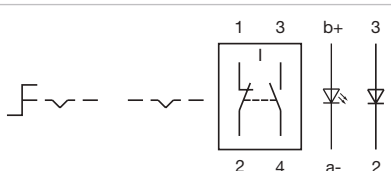
Wiring diagram 280
