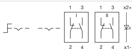
Wiring diagram 276
