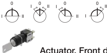
Actuator, Front dimension Ø 18 mm
