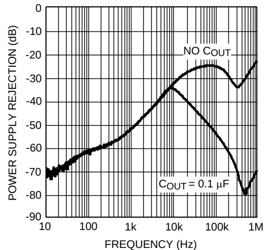
Figure 16. Power Supply Rejection vs Frequency
