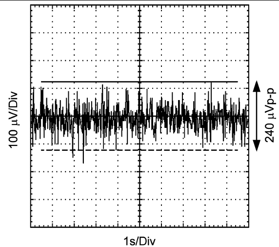
Figure 26. 0.1–10 Hz Noise
