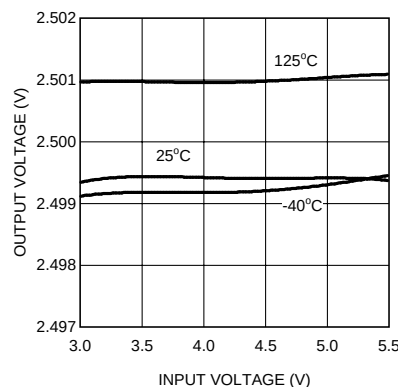
Figure 50. Line Regulation
