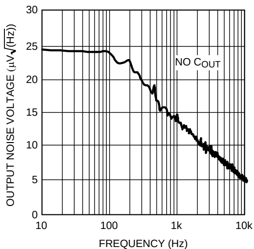
Figure 33. Output Voltage Noise Spectrum
