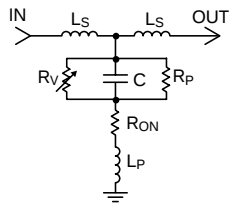
Electrical Model
