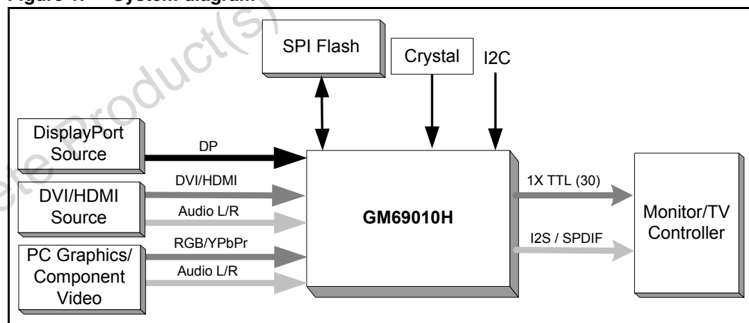
Figure 1. System diagram
