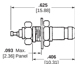
8-32 UNC-2A (Modified)
