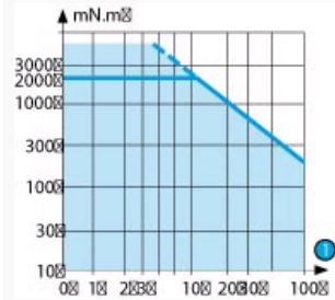
Curves : Curve: torque/nominal speed
