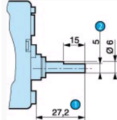
Dimension Diagram : Shaft 79202573
