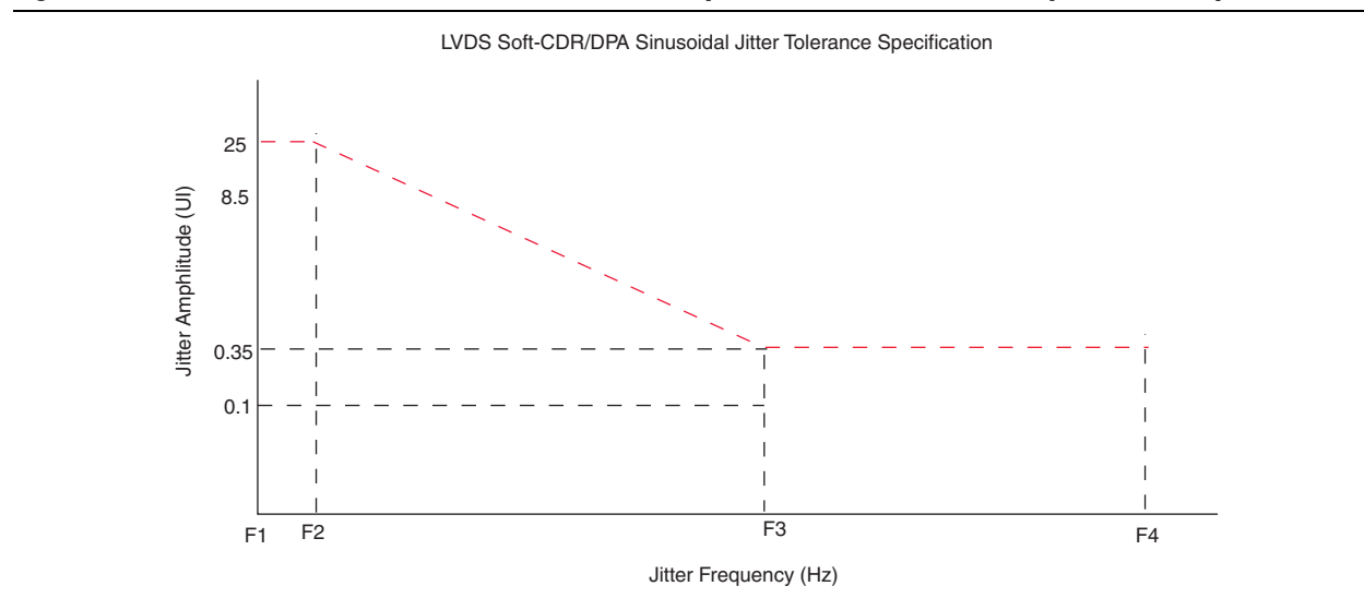
Figure 2-2. LVDS Soft-CDR/DPA Sinusoidal Jitter Tolerance Specification for a Data Rate Equal to 1.25 Gbps
