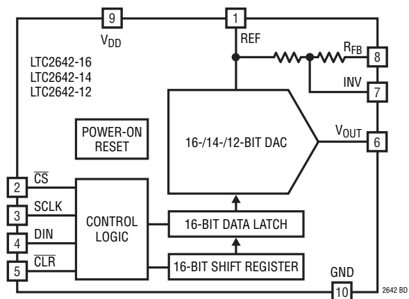
LTC2642
