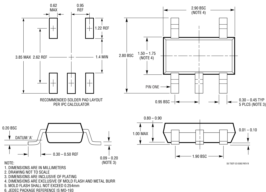
S5 Package 5-Lead Plastic TSOT-23 (Reference LTC DWG # 05-08-1635)
