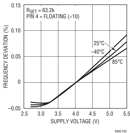
Figure 5. Supply Sensitivity
