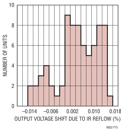
Figure 15. Output Voltage Shift Due to IR Reflow
