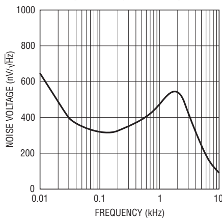
5V Output Voltage Noise Spectrum
