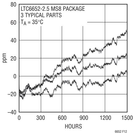
Figure 12. Long-Term Drift
