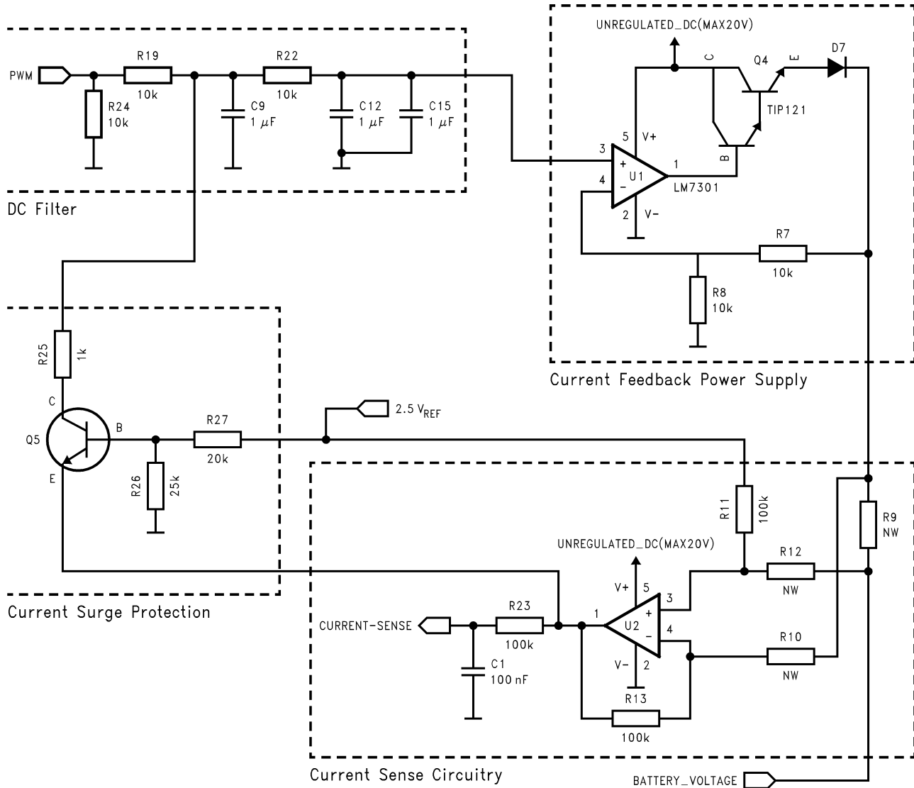
Figure 8. Circuitry Used for Li-Ion
