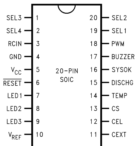
Figure 1. Top View See Package SOIC (DW)
