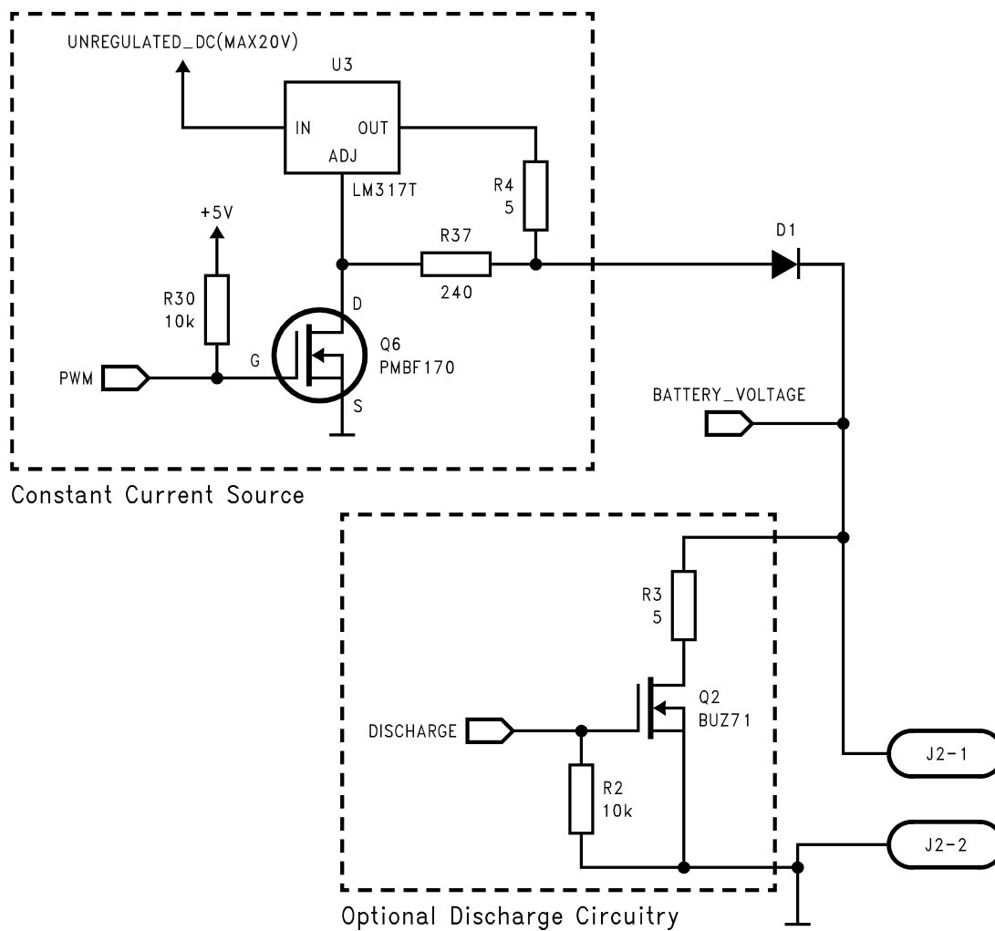
Figure 7. Circuitry Used Only for Ni-Cd/Ni-MH
