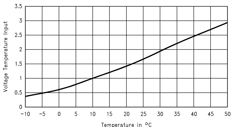
Figure 5. Typical Configuration Curve, (NTC Characteristics: 3 k \Omega @ 25°C, \beta=3988 )
