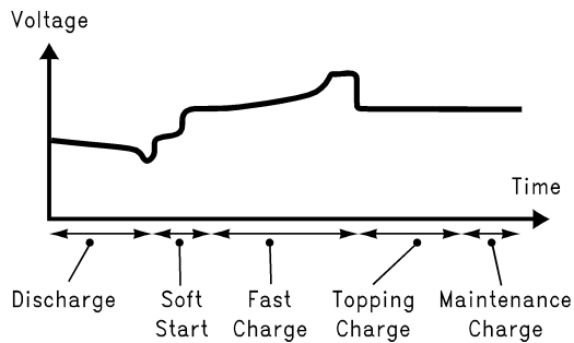
Figure 2. Ni-Cd Charging Curve
