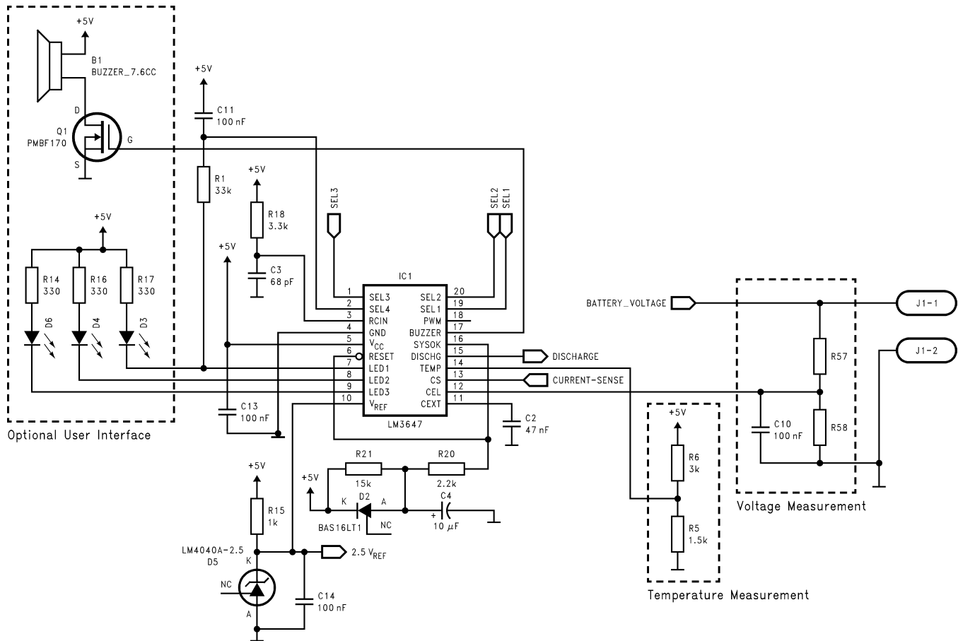
Figure 6. Common Circuitry Used for both Ni-Cd/Ni-MH and Li-Ion
