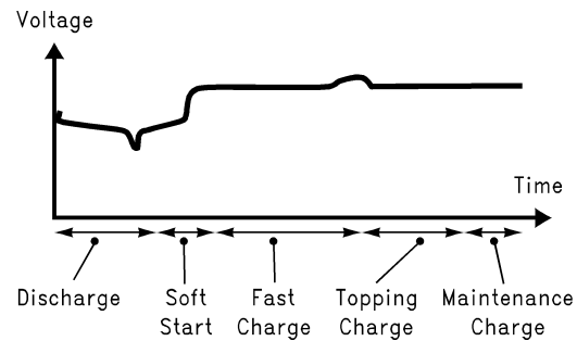
Figure 3. Ni-MH Charging Curve
