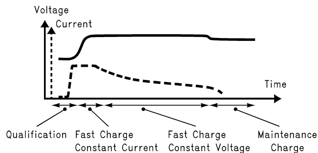
Figure 4. Li-Ion Charging Curve
