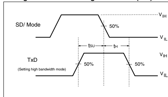
Figure 4. Bandwidth Programming
