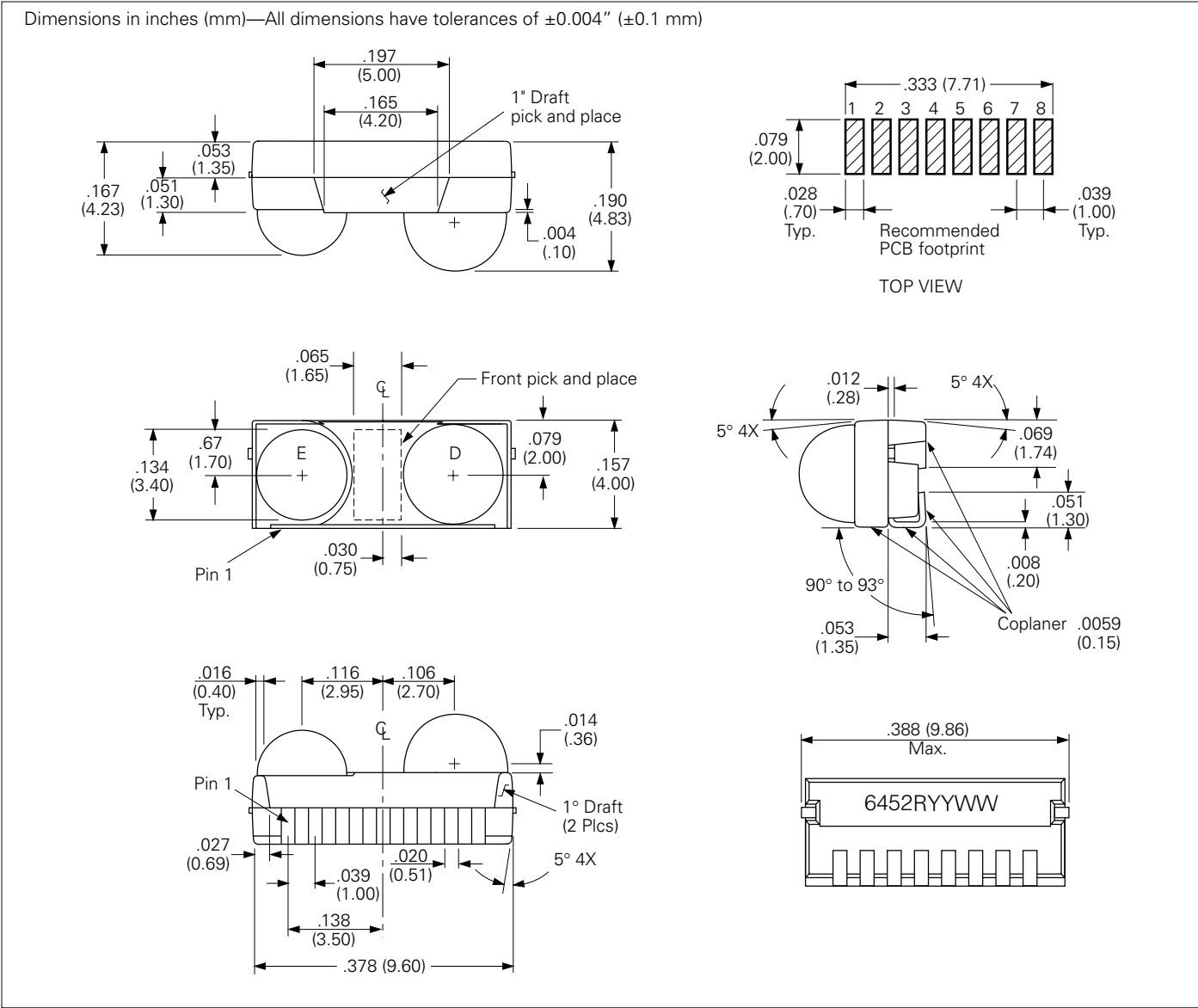
Figure 11. IRMS6452/IRMT6452 detail drawings with optional side view or top view mounting
