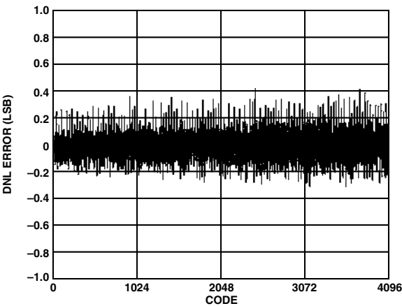
TPC 4. Typical DNL For the AD7453 for V_{DD} = 5\text{ V}
