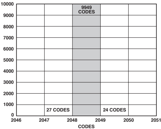
TPC 6. Histogram of 10,000 Conversions of a DC Input
