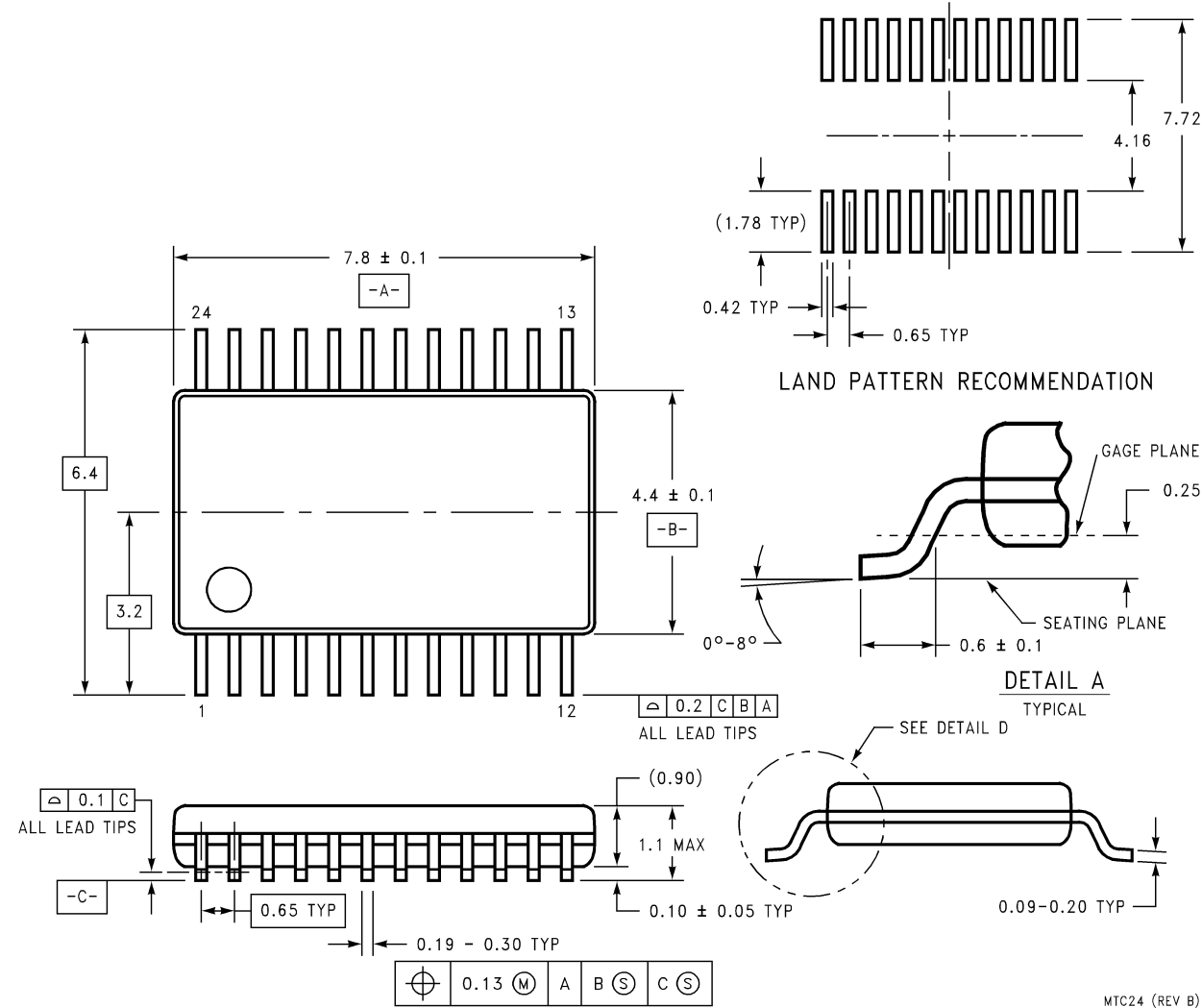
24-Lead TSSOP Order Number LM81BIMT-3, LM81BIMTX-3, LM81CIMT-3 or LM81CIMTX-3 NS Package Number MTC24B
