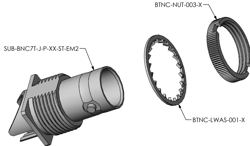
FIG 1 BNC7T-J-P-XX-ST-EM2 SHOWN
