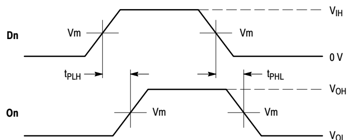
WAVEFORM 1 - PROPAGATION DELAYS t_R = t_F = 2.0 ns, 10% to 90%; f = 1 MHz; t_W = 500 ns Figure 4. AC Waveforms
