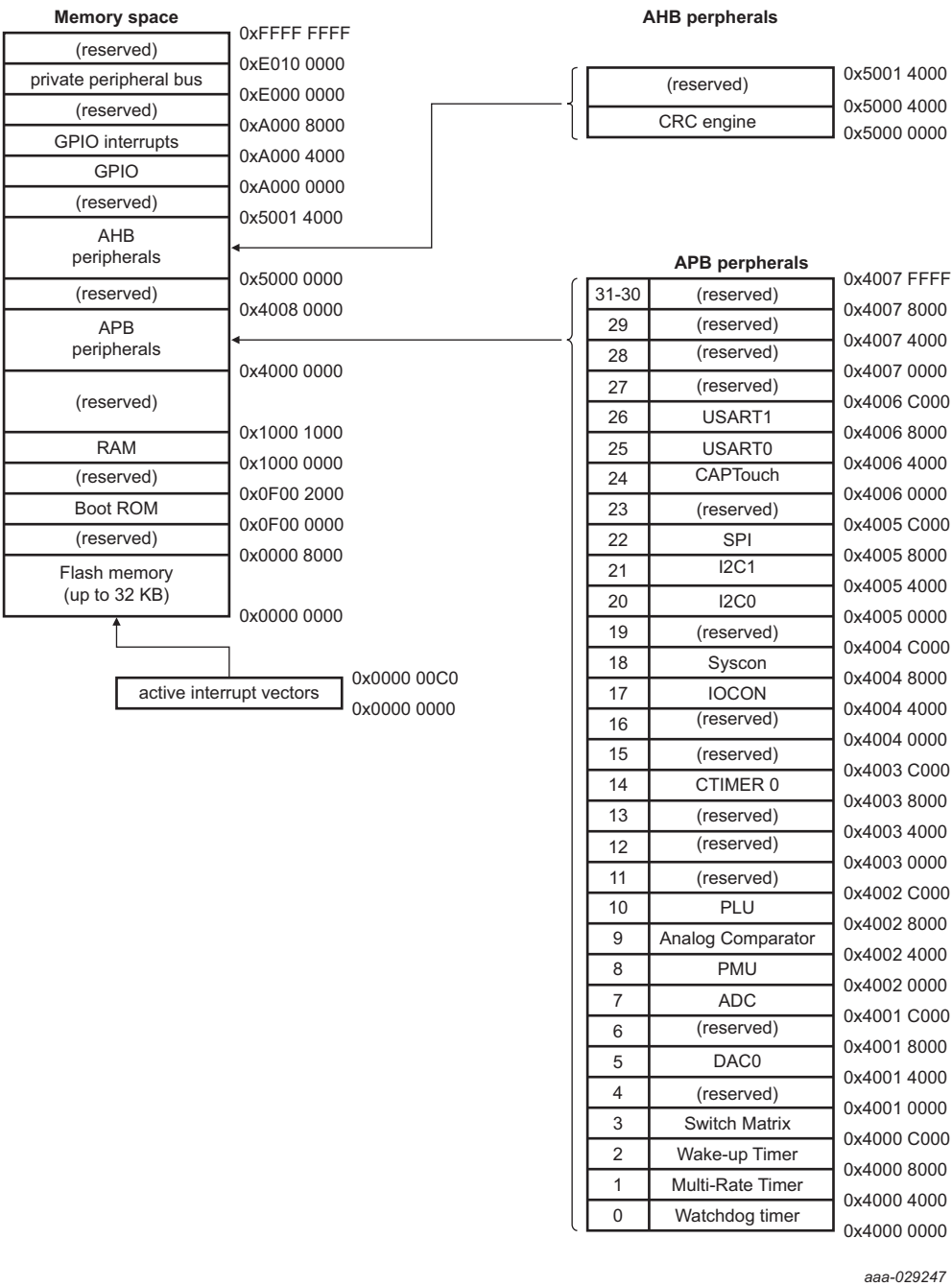
Fig 9. LPC804 Memory mapping
