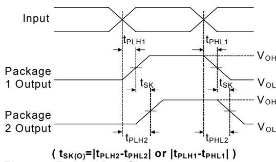
Figure 5. Part-to-Part Skew
