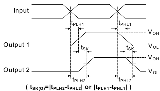
Figure 3. Output Skew
