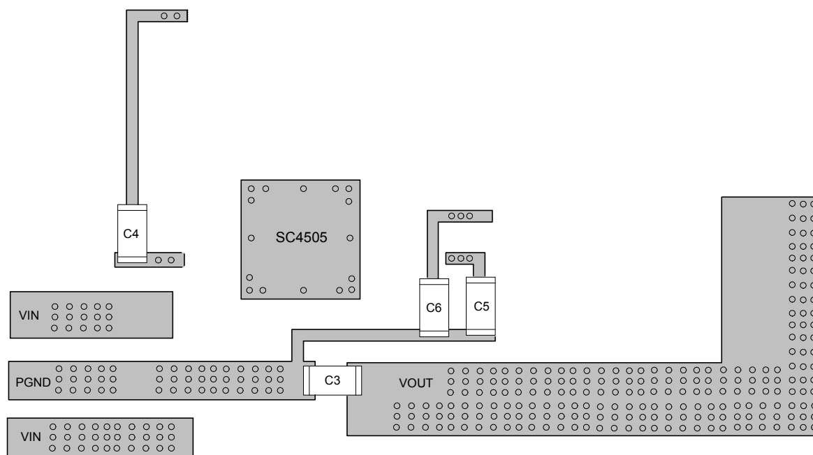
Figure 6b Layout Illustration -- Bottom Layer
