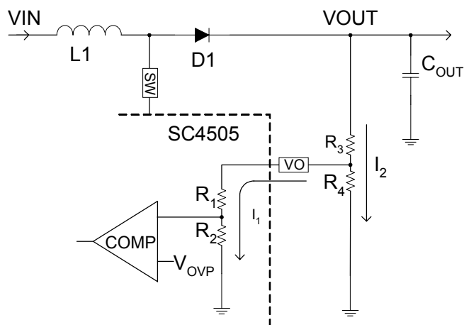
Figure 5. OVP Tweak
